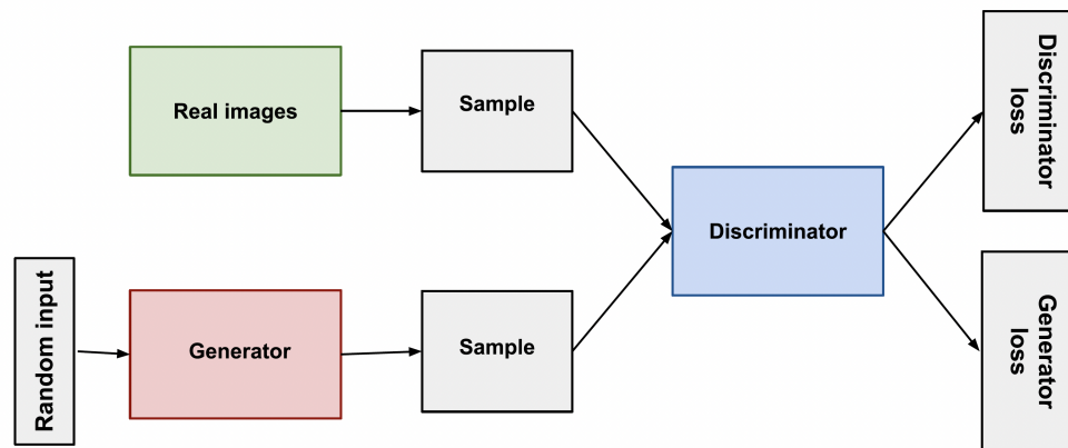
The basic structure of a GAN. Source: Google
